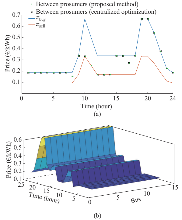
Fig. 3. Energy prices with connected feeders (case 2). (a) Profiles of prices of transaction with utility grid and energy prices of exchanges between prosumers. (b) Energy prices of exchanges between prosumers at different buses.
