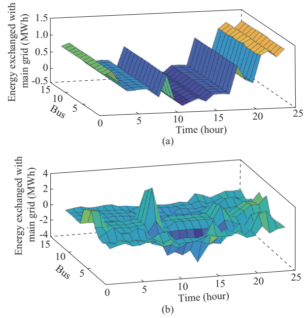
Fig. 7. Energy exchanged with main grid for 14-bus distribution network. (a) With P2P energy exchanges among prosumers (case 2). (b) Without energy exchanges among prosumers (case 1).
