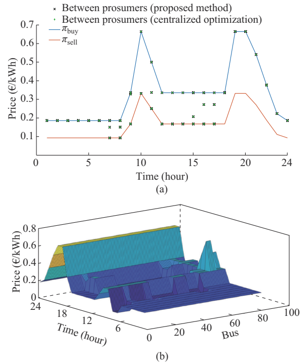
Fig. 12. Energy prices with separated feeders (case 3) for 81-bus distribution network. (a) Profiles of prices of transactions with utility grid and energy prices of exchanges between prosumers. (b) Energy prices of exchanges between prosumers at different buses.
