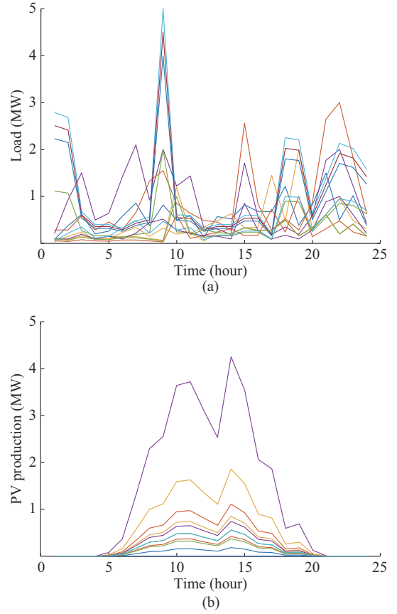
Fig. 2. Prosumer characteristics for 14-bus distribution network. (a) Load profiles. (b) PV production profiles for each prosumer.
