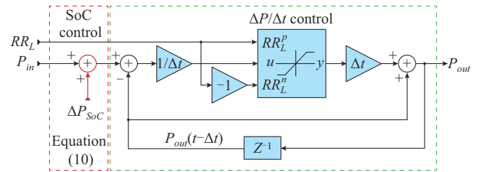
Fig. 4. Main control block for producing smoothed active power profile.
