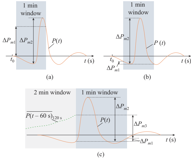
Fig. 1. Power variation computation for a 1 min window according to three definitions. (a) \Delta P_{m1} ( t=t_0 ). (b) \Delta P_{m2} ( t=t_0 + 20 s). (c) \Delta P_{m3} ( t=t_0 + 40 s).
