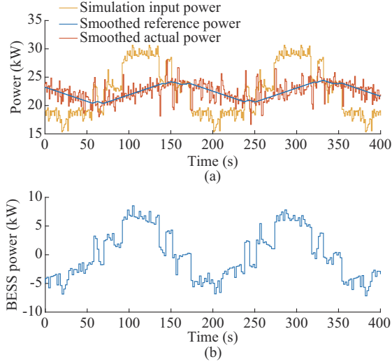
Fig. 7. Validation of RR control through simulations. (a) Simulation input power, smoothed reference power, and smoothed actual power. (b) BESS power.
