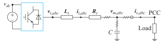
Fig. 1. One-line diagram of an LC-coupled VSC connected to an islanded system.
