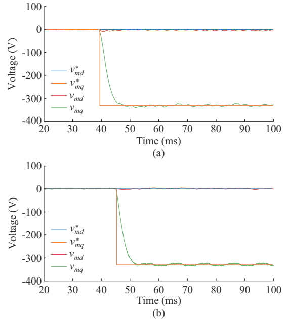
Fig. 10. Voltages in dq coordinates for transient behaviour. (a) Three-phase delta resistive balanced load of 42 \Omega per phase. (b) No-load operation.
