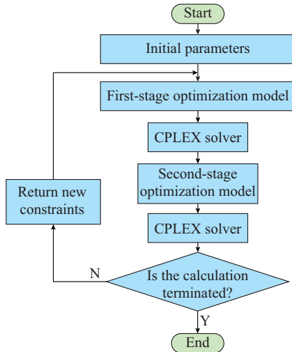
Fig. 2. Solution process of robust optimization model.
