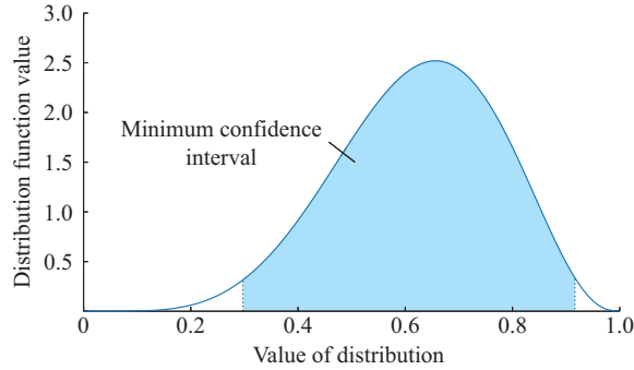
Fig. 6. Beta distribution and minimum confidence interval.
