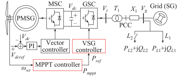
Fig. 2. Equivalent model of power grid with WFs.
