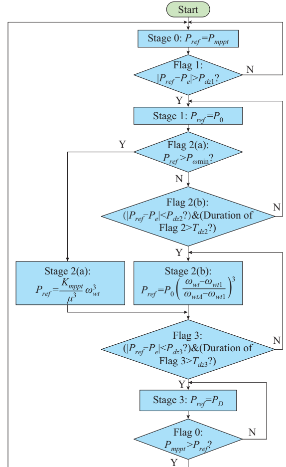
Fig. 8. Flowchart of proposed scheme.
