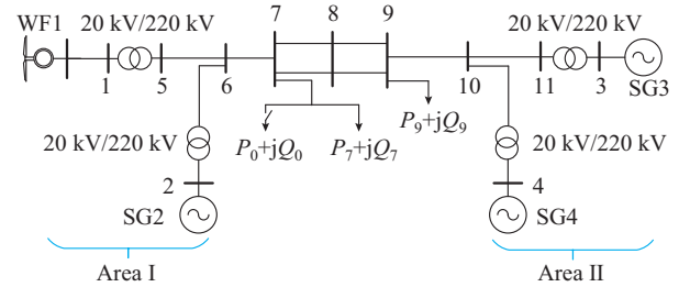
Fig. 15. Simulation model of IEEE 4-machine 2-area system.
