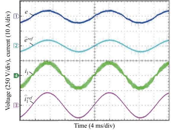
Fig. 8. Steady-state control voltage, estimated voltage reference, inverter-side current, and inverter-side current reference, with proposed controller (including harmonic compensation) and considering P_{ref}=700 W.
