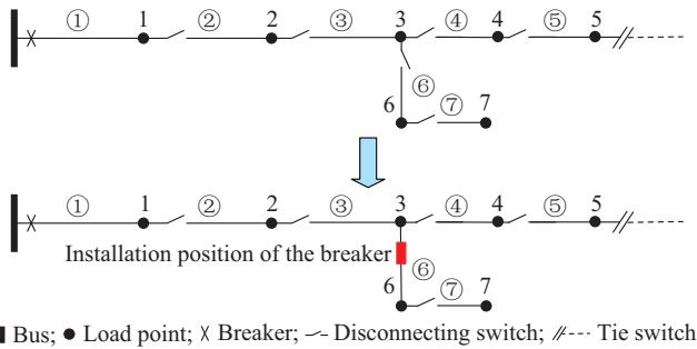
Fig. 4. Installation position of an added circuit breaker.
